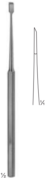
06-8297 4mm FREER Chisel 160 mm
